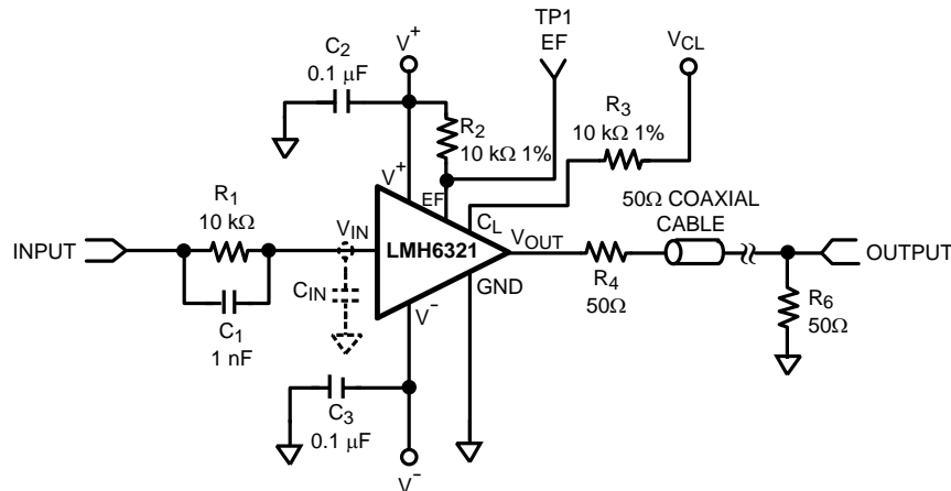
Figure 52. 50Ω Coaxial Cable Driver with Dual Supplies
