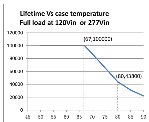
Life Time VS. Tcase (Ref.)(Model:6.8A)
