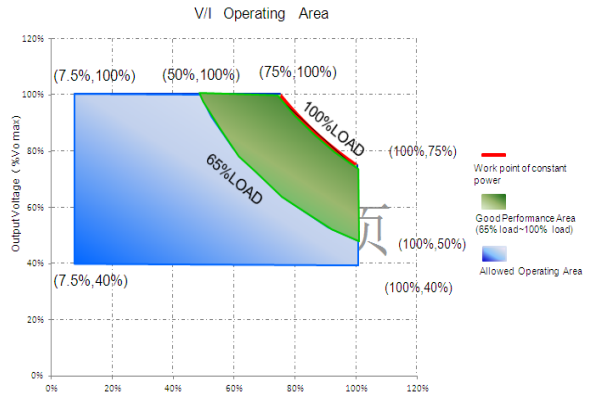
V/I Curve
