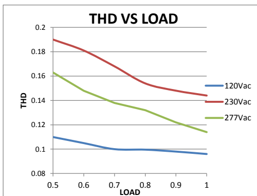
THD VS. Load Curve(Model:6.8A)
