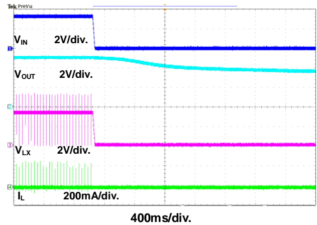
Figure 9. Power Off through VIN Waveform
