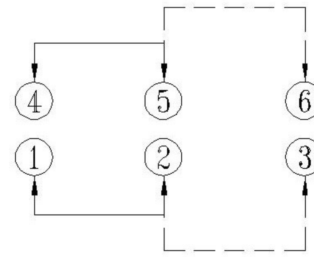
SCHEMATIC (NON-SHORTING)
