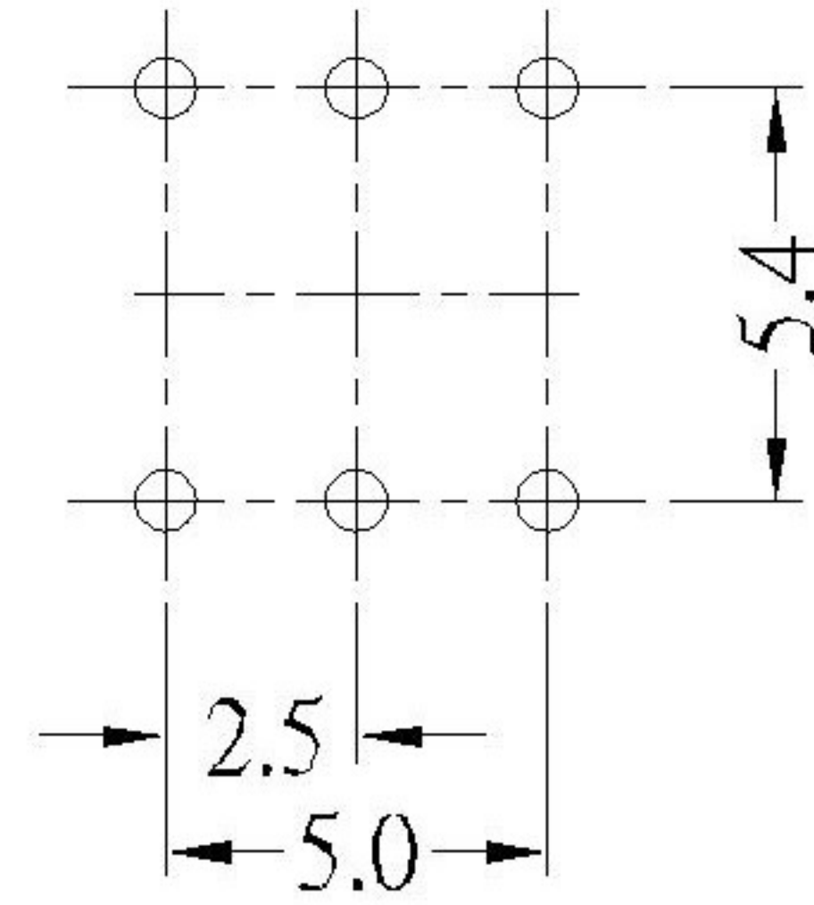
P.C.B LAYOUT BOTTOM VIEW
