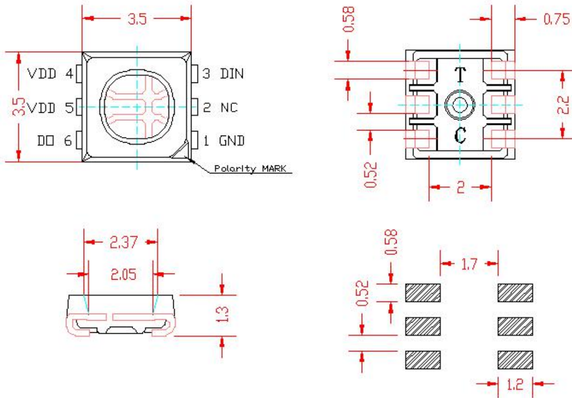
Recommended size of solder pad
