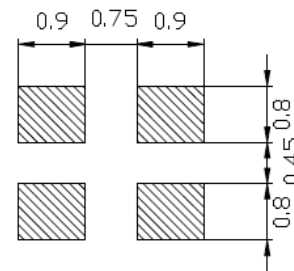
LAND PATTERN<REFERENCE>
