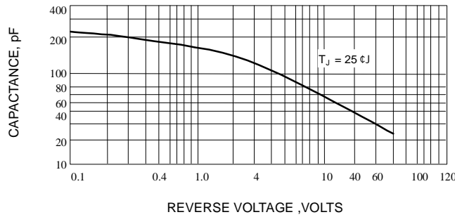
Fig. 4-TYPICAL JUNCTION CAPACITANCE
