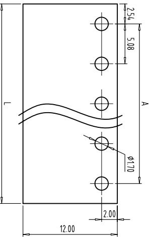
PCB LAYOUT S=2.5:1
