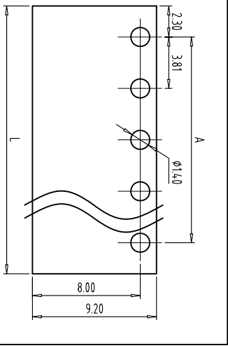
PCB LAYOUT S=3:1
