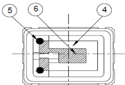
A-A' sectional drawing
